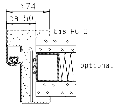
Zarge "ZG 68/76"
