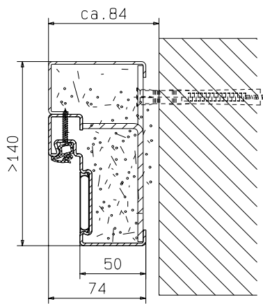
Zarge "ZNG 68/76"
