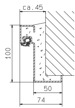
Hauptzarge "ZG 68/76"
