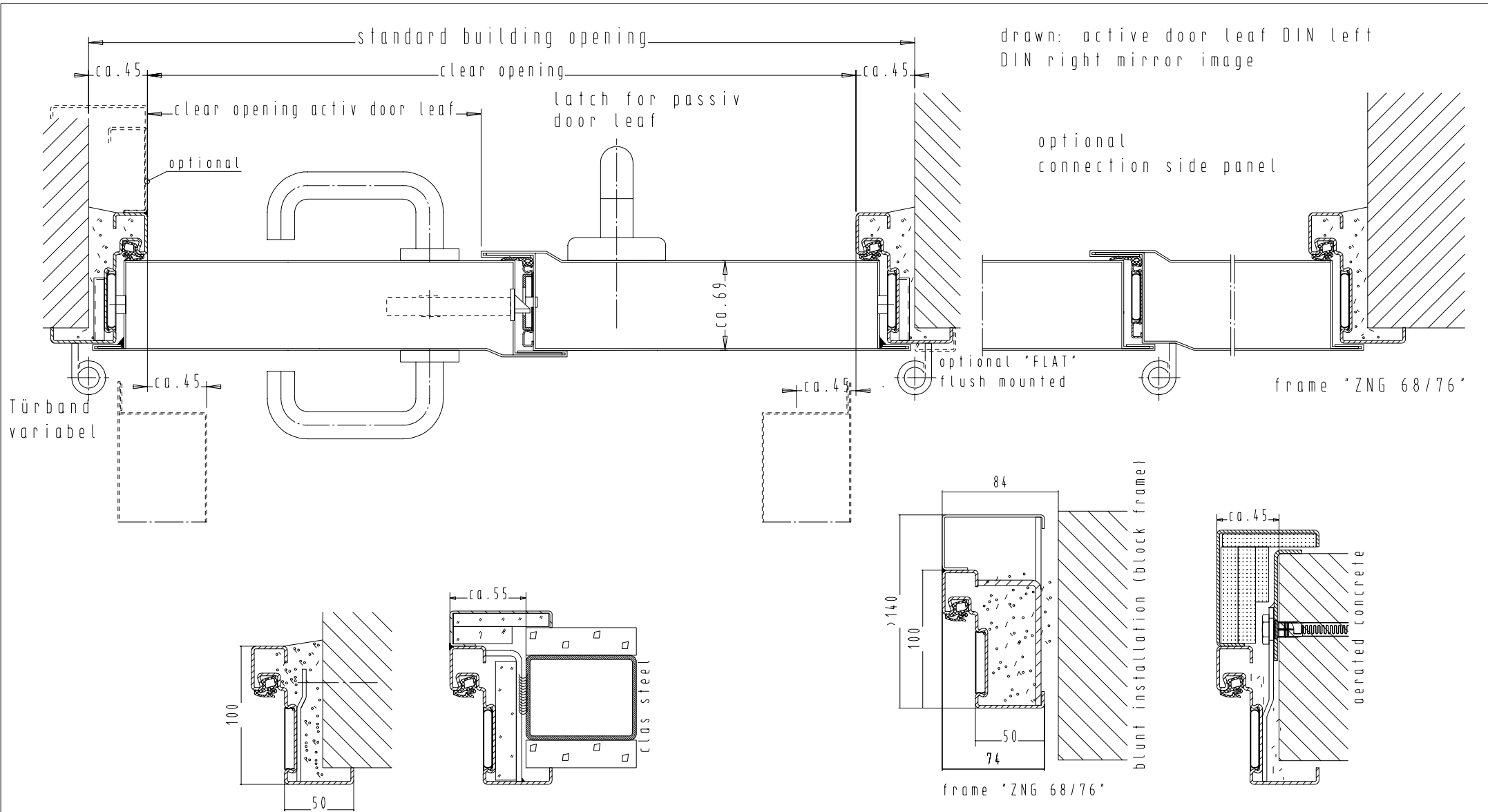
frame "ZNG 68/76"
